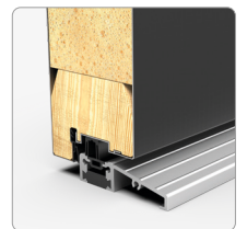
4 sides rebated Low, aluminium threshold with thermal break
